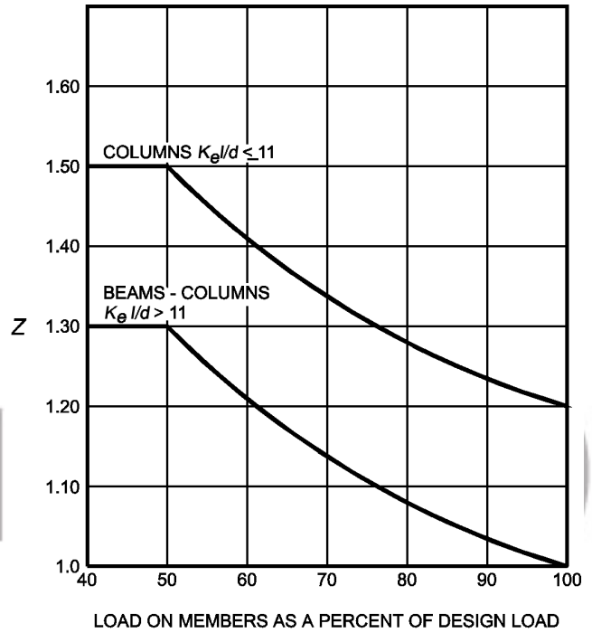
FIGURE 721.6.3(1) LOAD FIGURE
