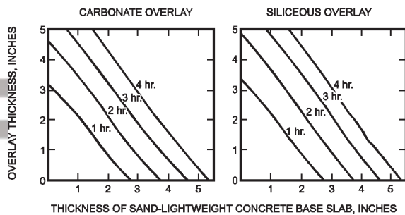
FIGURE 721.2.2.2 FIRE-RESISTANCE RATINGS FOR TWO-COURSE
