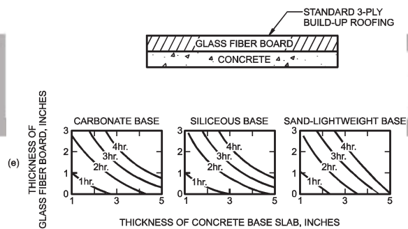
FIGURE 721.2.2.3(2) FIRE-RESISTANCE RATINGS FOR CONCRETE ROOF ASSEMBLIES
