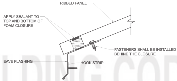
FIGURE 2 TYPICAL EAVE TERMINATION DETAIL WITH CLOSURE STRIP
