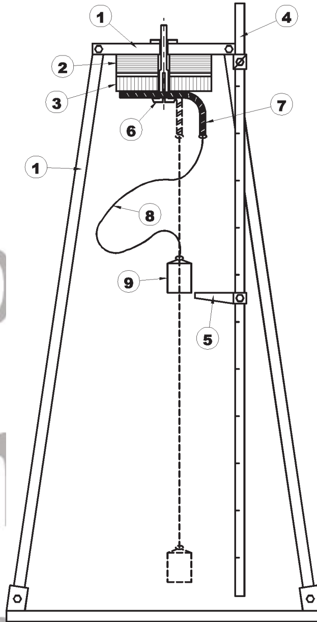
FIGURE 1 DIAGRAM OF DYNAMIC PULL-OFF TEST APPARATUS
