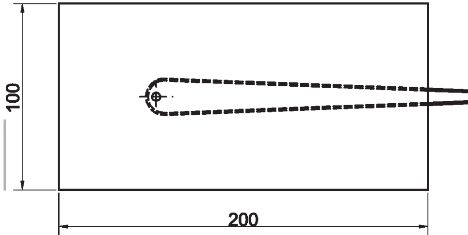
FIGURE 2 DIAGRAM OF WIRE REINFORCED TEST STRAP
