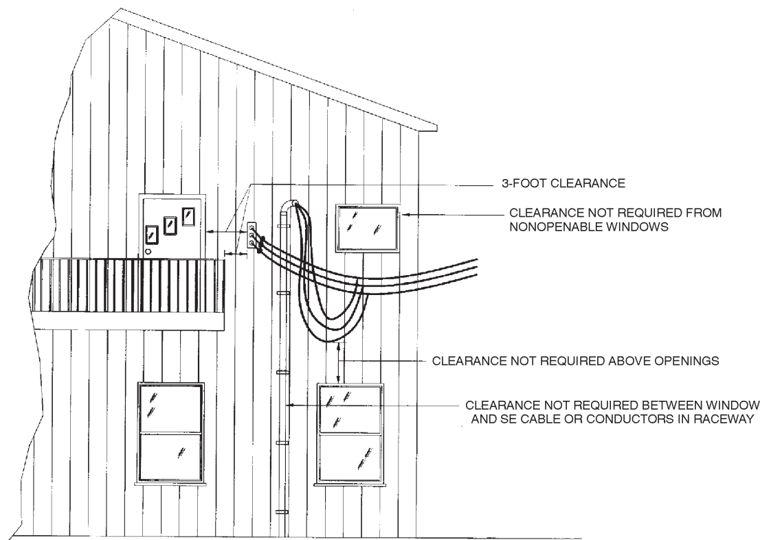
FIGURE E3504.1 [230.9] CLEARANCES FROM BUILDING OPENINGS
