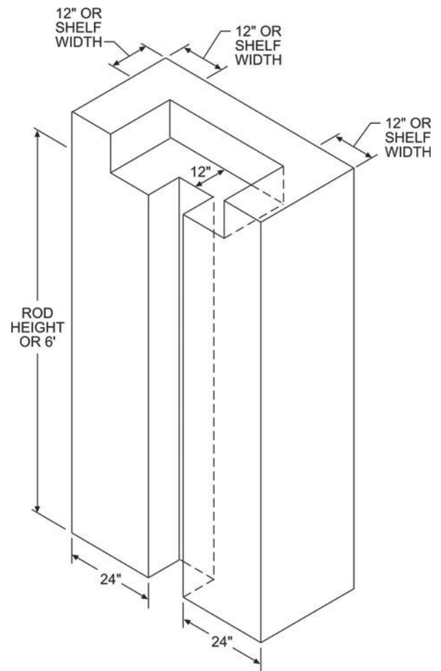
FIGURE E3903.11 [FIGURE 410.8] CLOSET STORAGE SPACE
