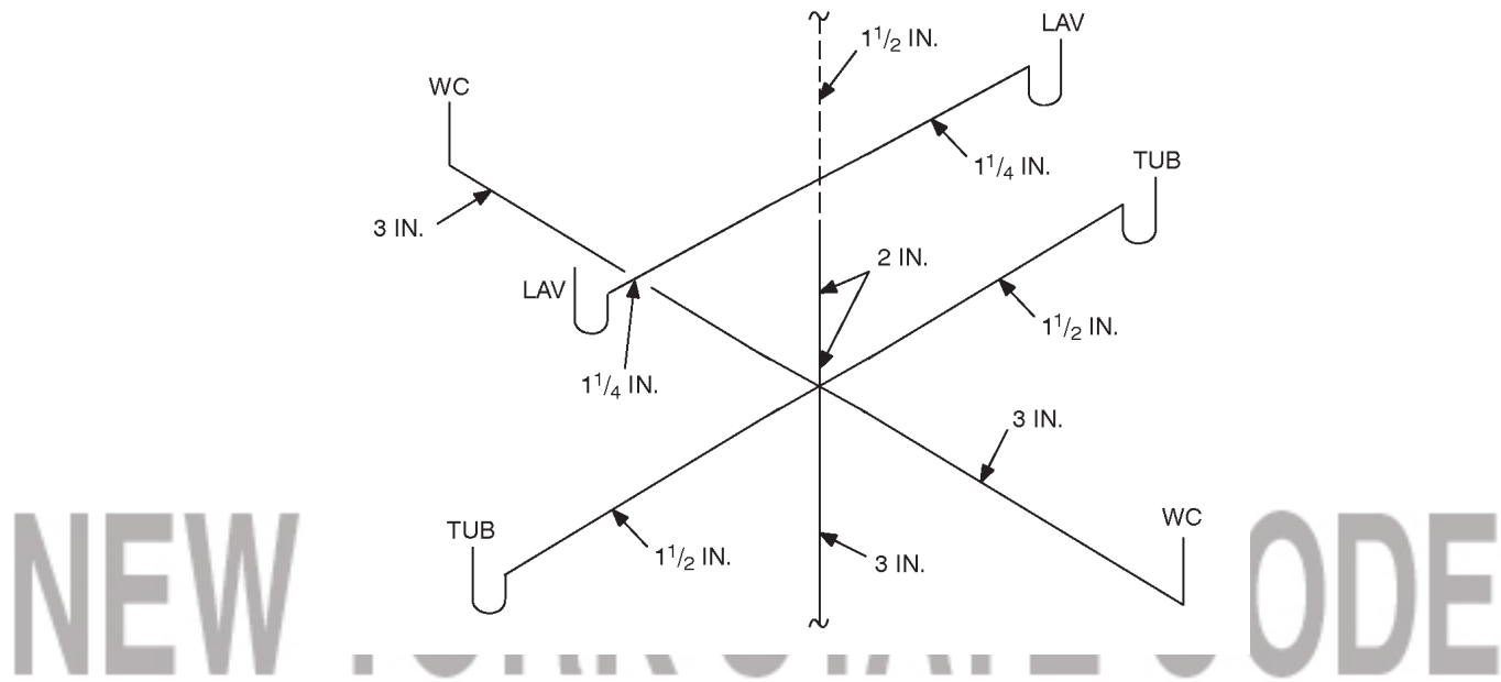
A. VERTICAL WET VENTING
