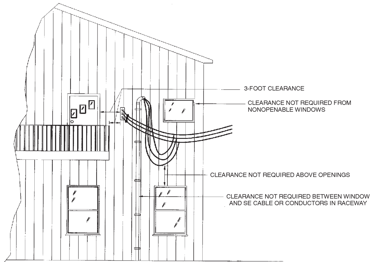
FIGURE E3504.1 CLEARANCES FROM BUILDING OPENINGS
