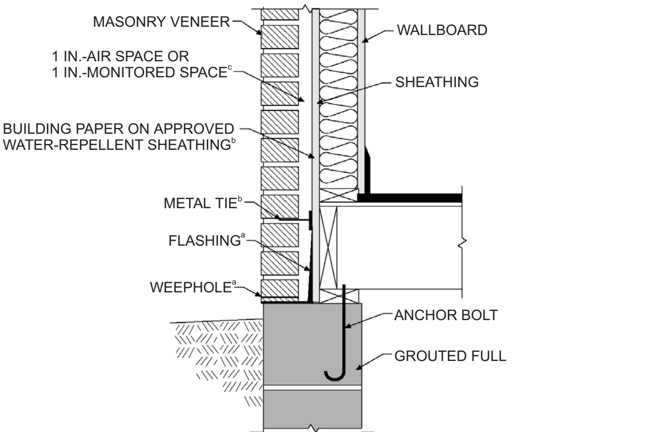
FIGURE R703.7 MASONRY VENEER WALL DETAILS (continued)
