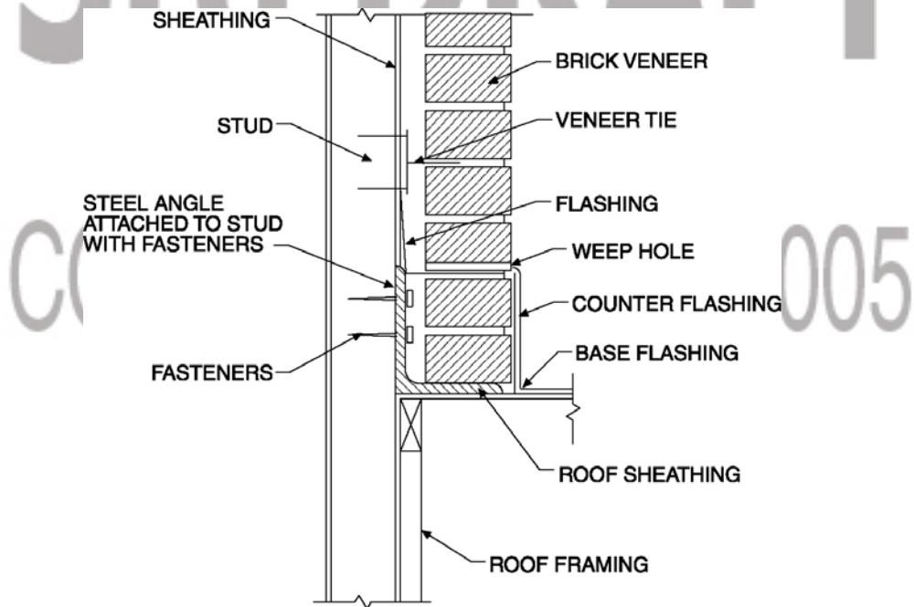
SUPPORT BY STEEL ANGLE
