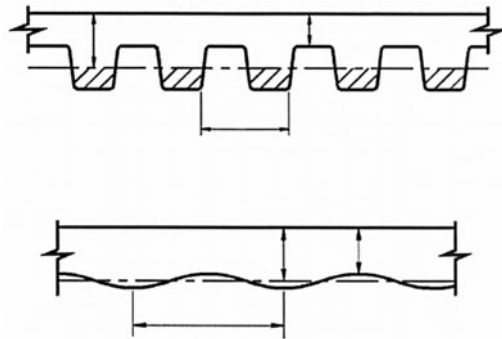
FIGURE 721.2.2.1.3 SLABS WITH RIBBED OR UNDULATING SOFFITS
