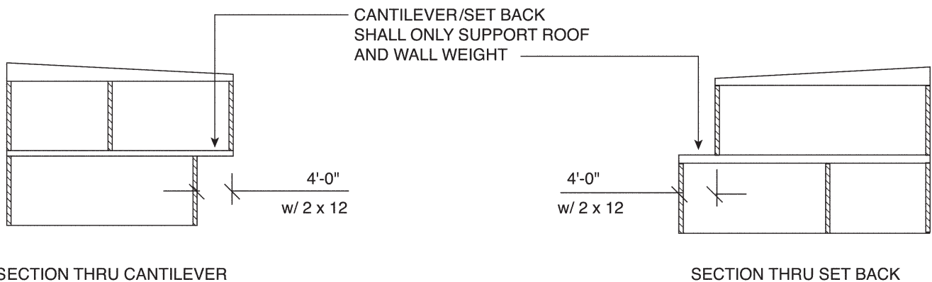
FIGURE 2308.12.6(1) BRACED WALL PANELS OUT OF PLANE
