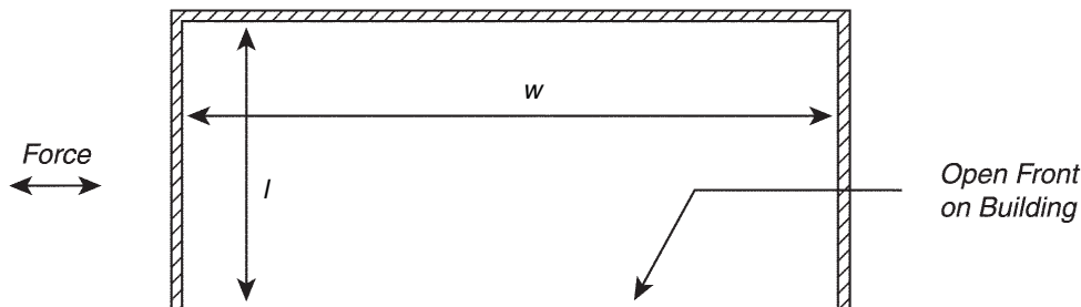
FIGURE 2305.2.5(1) DIAPHRAGM LENGTH AND WIDTH FOR PLAN VIEW OF OPEN FRONT BUILDING
