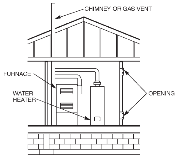
FIGURE G2407.5.3 ALL AIR FROM INSIDE THE BUILDING (see Section 2407.5.3)
