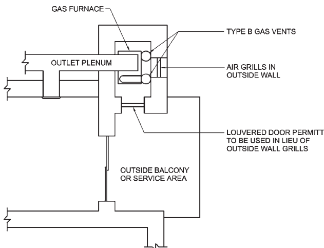
FIGURE C503.6.10.1 PLAN VIEW OF PRACTICAL SEPARATION METHOD FOR MULTISTORY GAS VENTING
