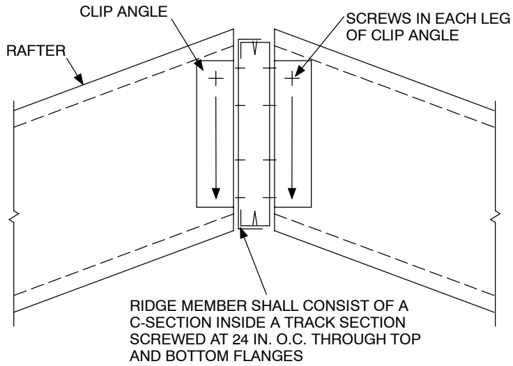
FIGURE R804.3.3.1 RIDGE BOARD CONNECTION
